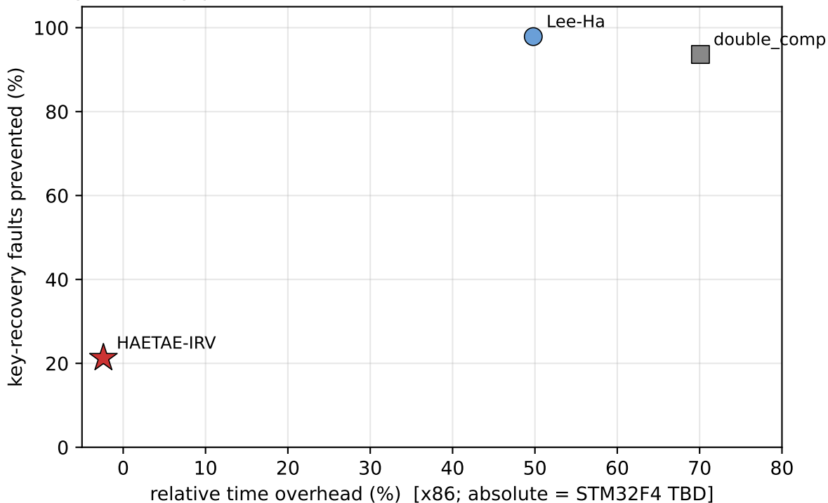
Key-recovery prevention vs overhead (IRV vs Lee-Ha, not combined)
