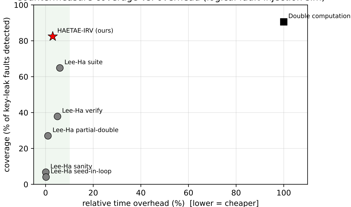
Countermeasure coverage vs. overhead (logical fault-injection sim)
