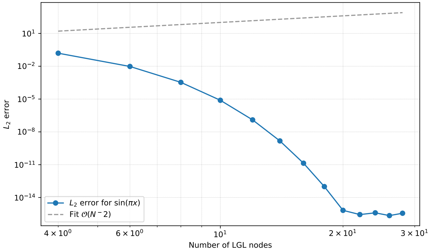
Legendre interpolation of \sin(\pi x)
