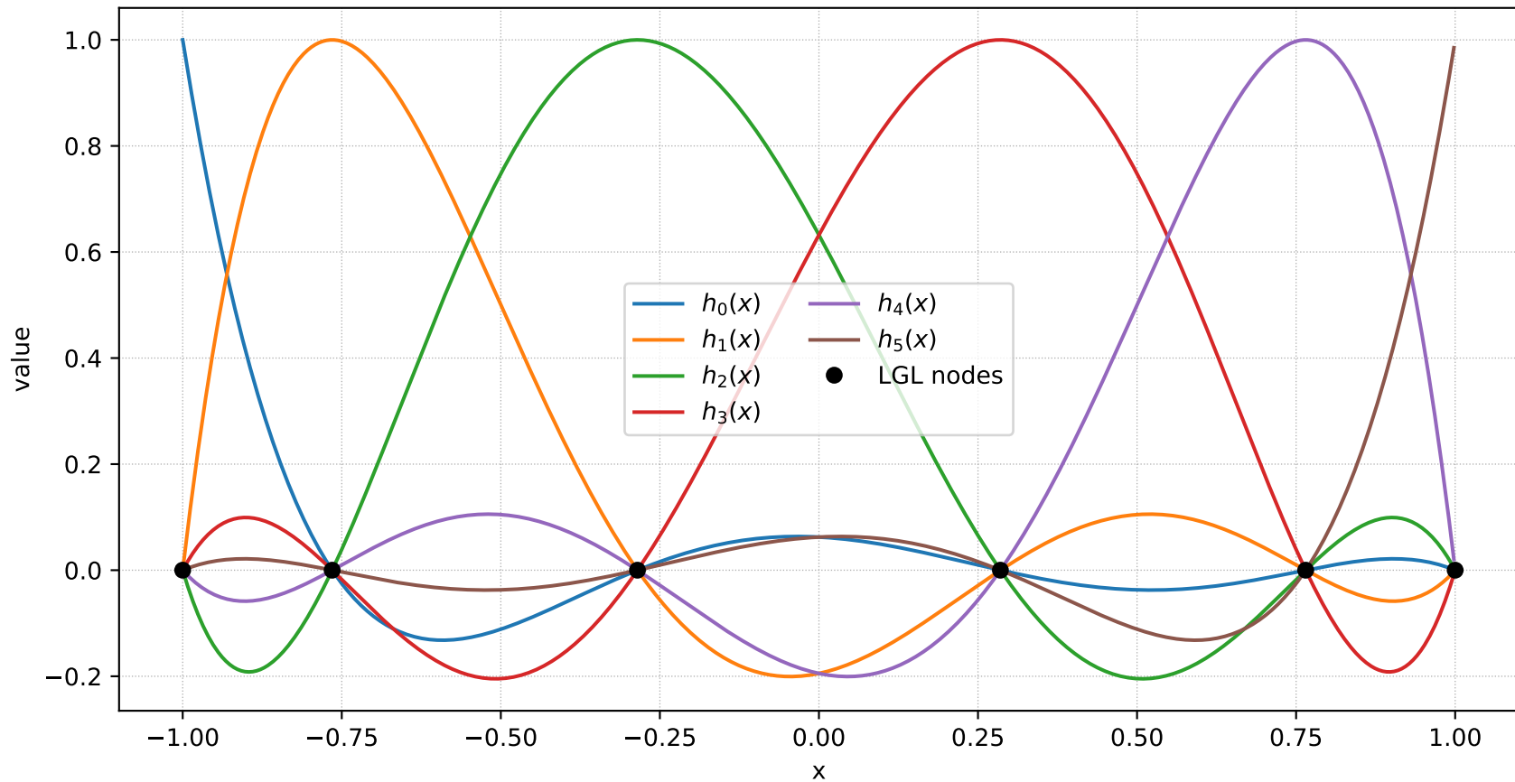
Legendre-Gauss-Lobatto Lagrange polynomials (N=6)
