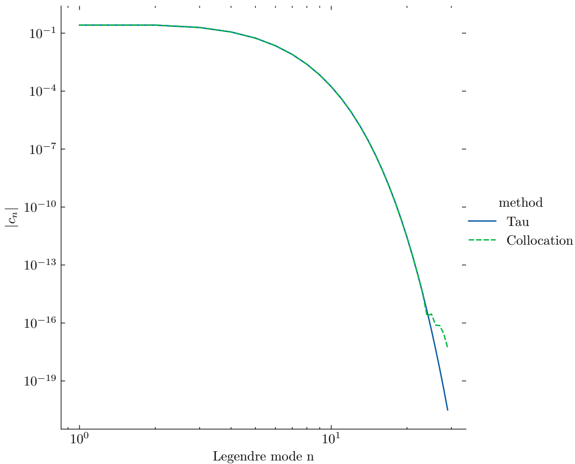
Coefficient decay, \epsilon = 0.1
