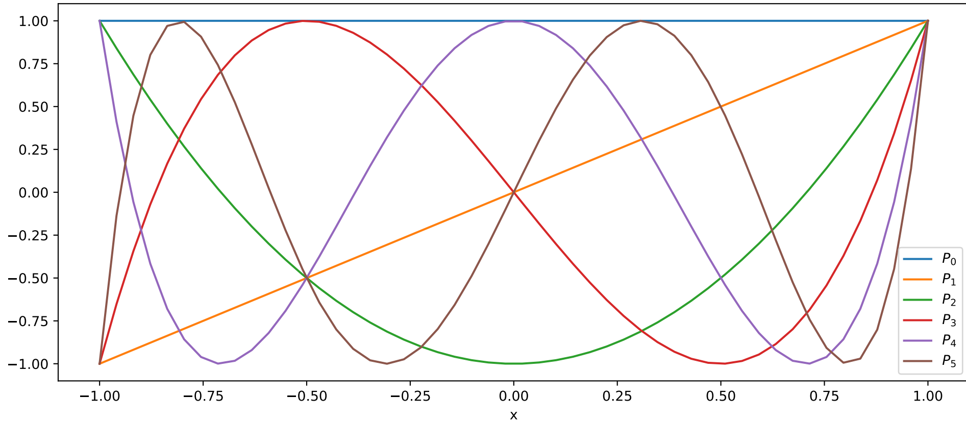
Chebyshev polynomials
