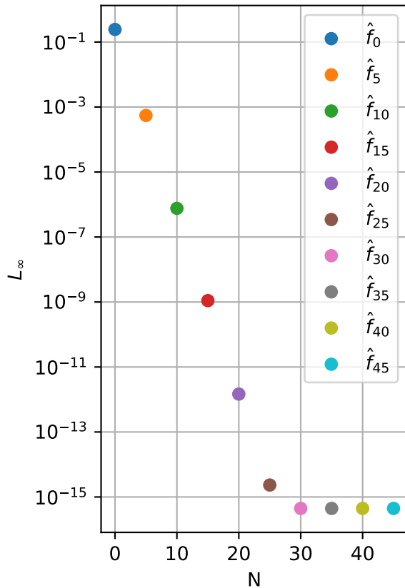
L_\infty error as a function of N
