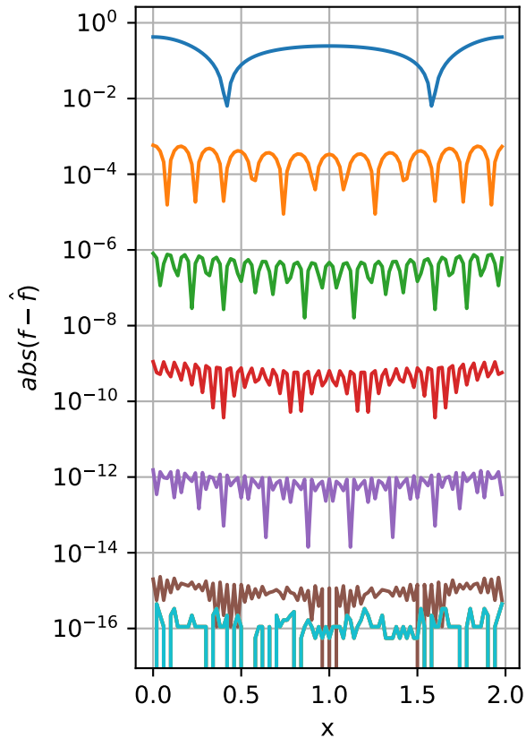
L_1 error as a function of x
