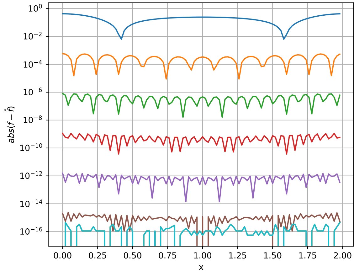
L_1 error as a function of x
