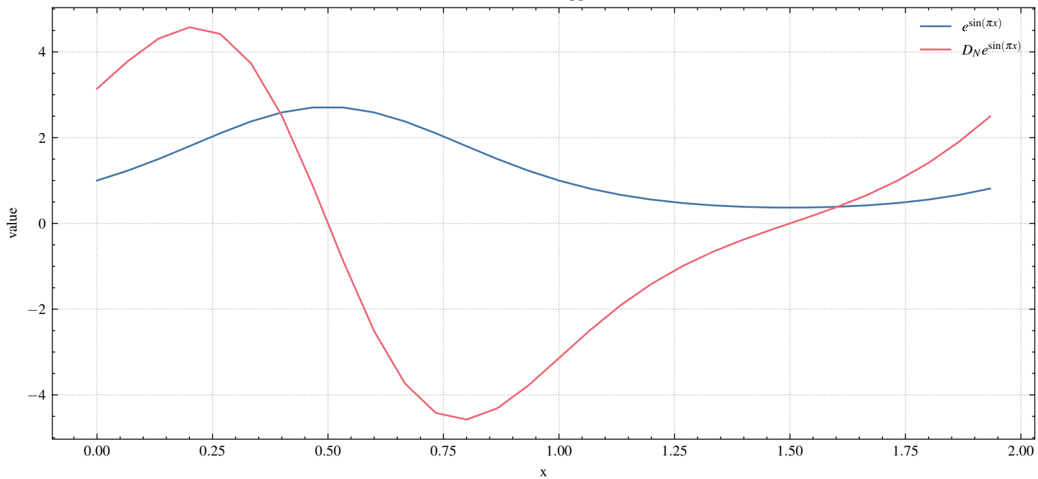
Differentiation matrix applied to e^{\sin(\pi x)}
