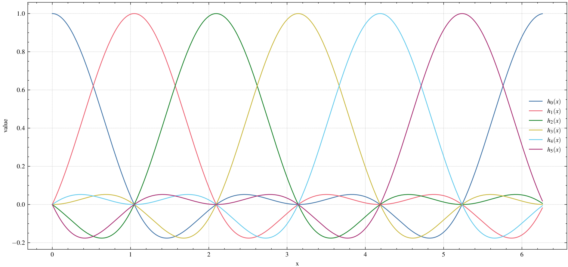
Fourier Lagrange polynomials on [0, 2\pi) (N=6)
