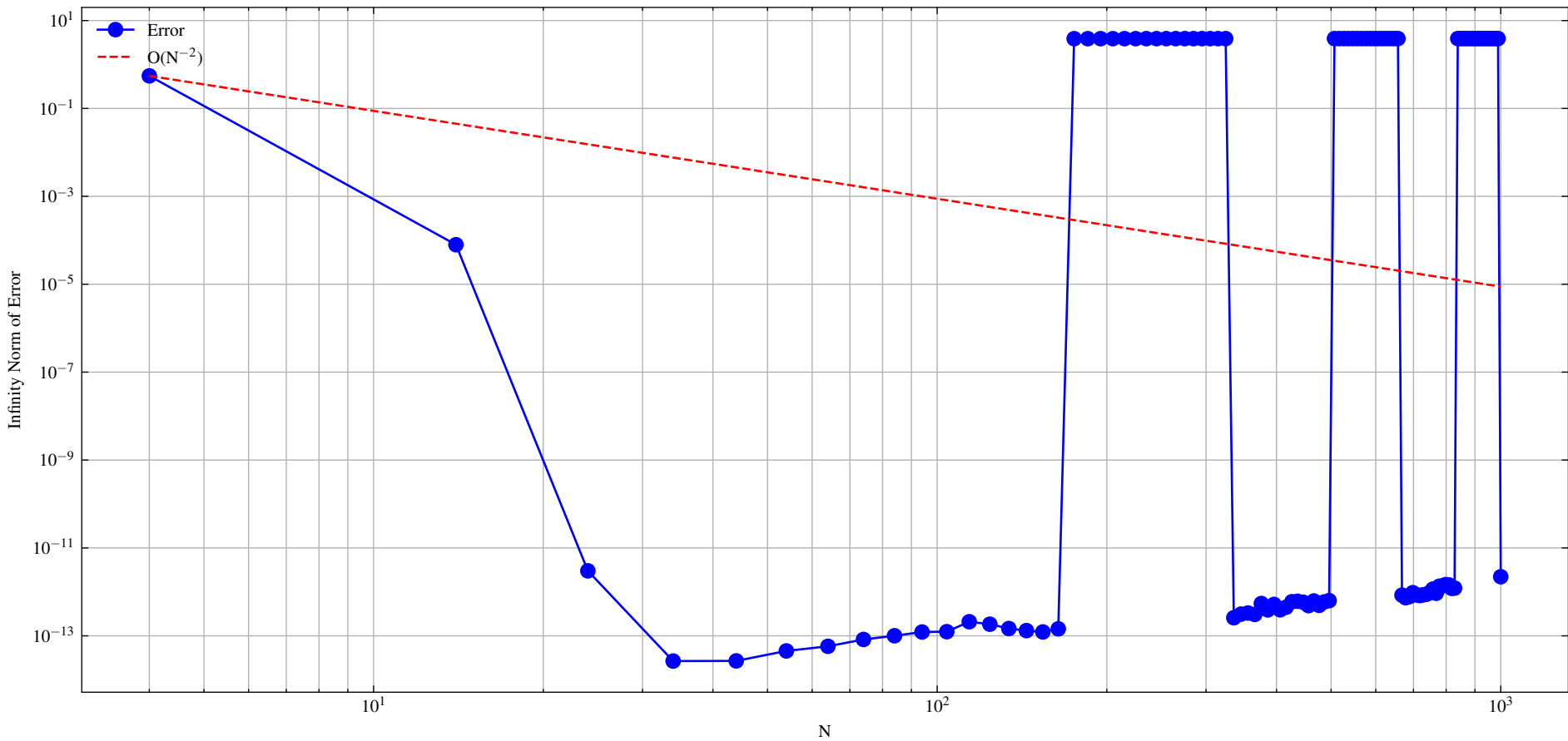
Convergence Rate of Fourier Spectral Differentiation
