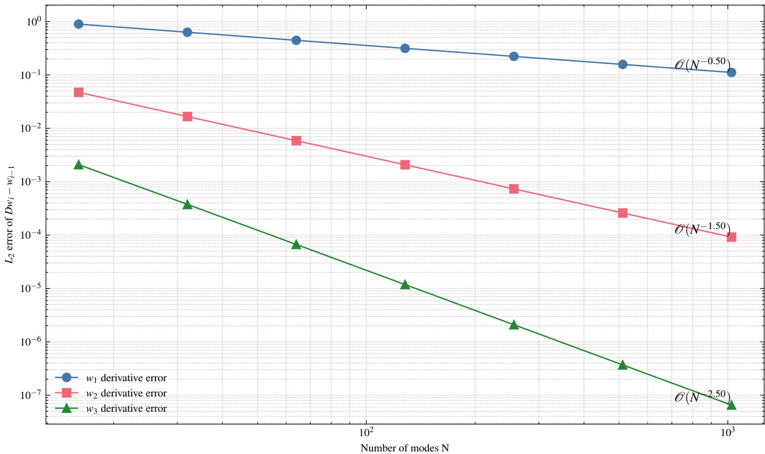
Fourier differentiation errors vs. grid resolution
