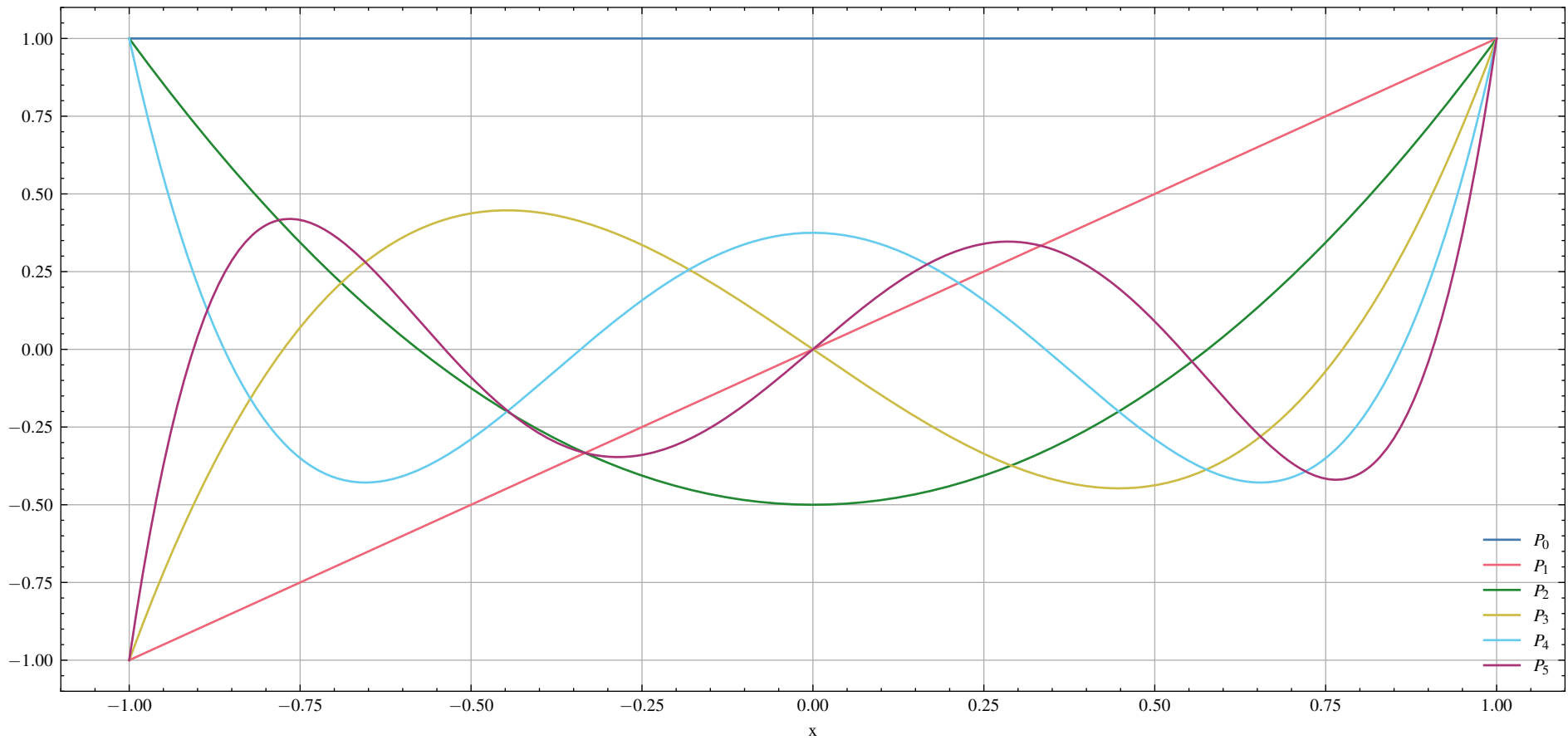
Legendre polynomials
