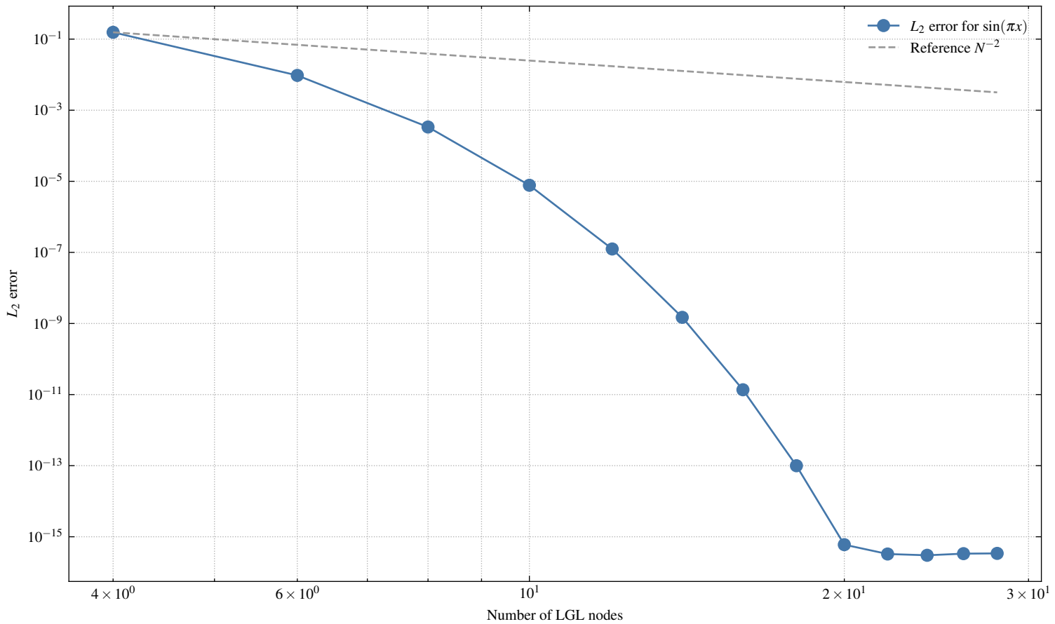
Legendre interpolation of \sin(\pi x)
