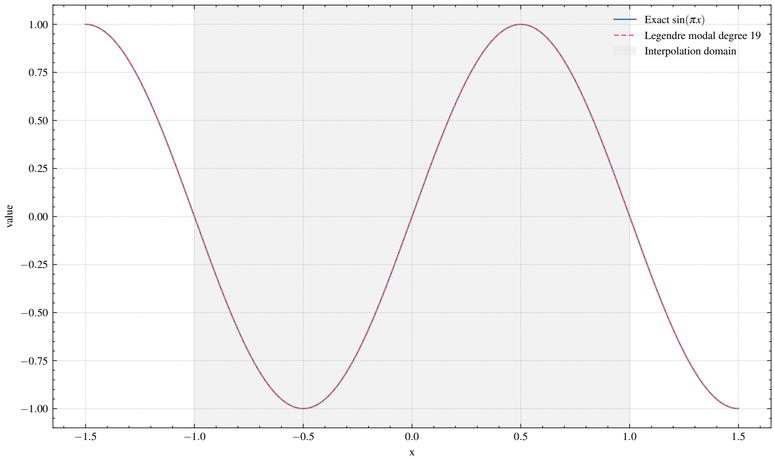
Legendre polynomial extrapolation
