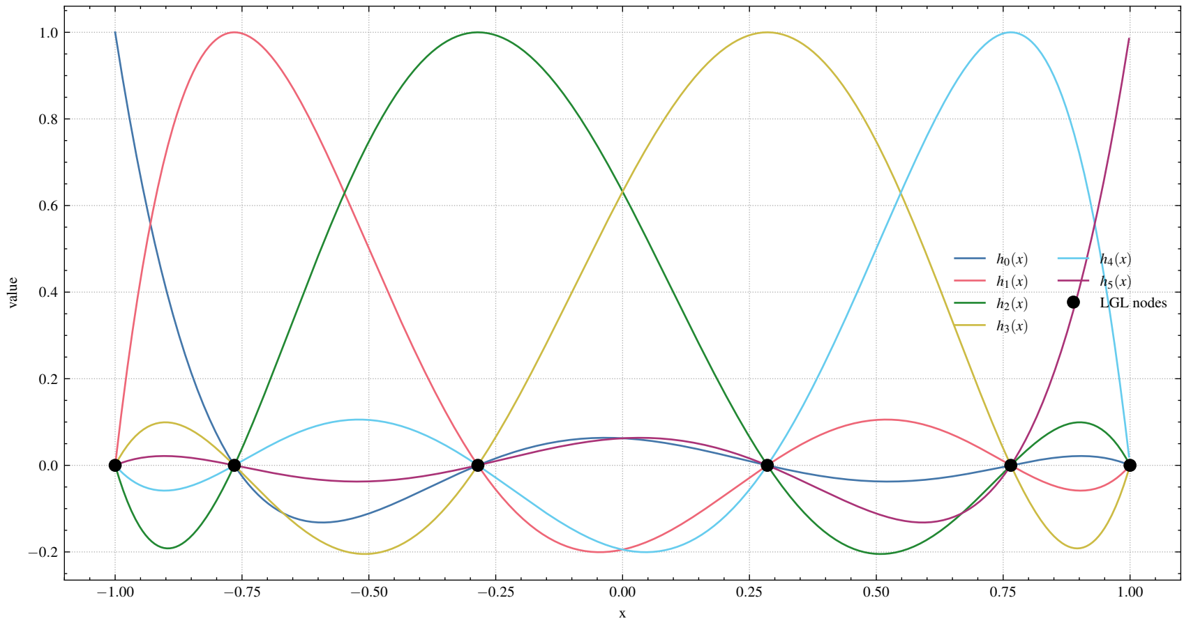
Legendre-Gauss-Lobatto Lagrange polynomials (N=6)
