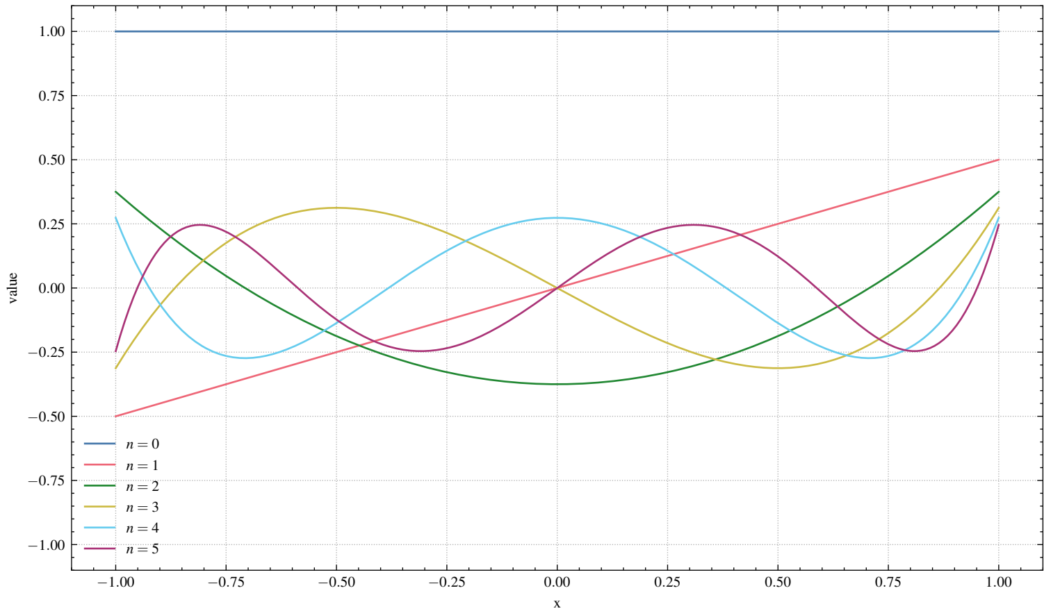
Jacobi polynomials (Chebyshev) P_n^{(-1/2,-1/2)}
