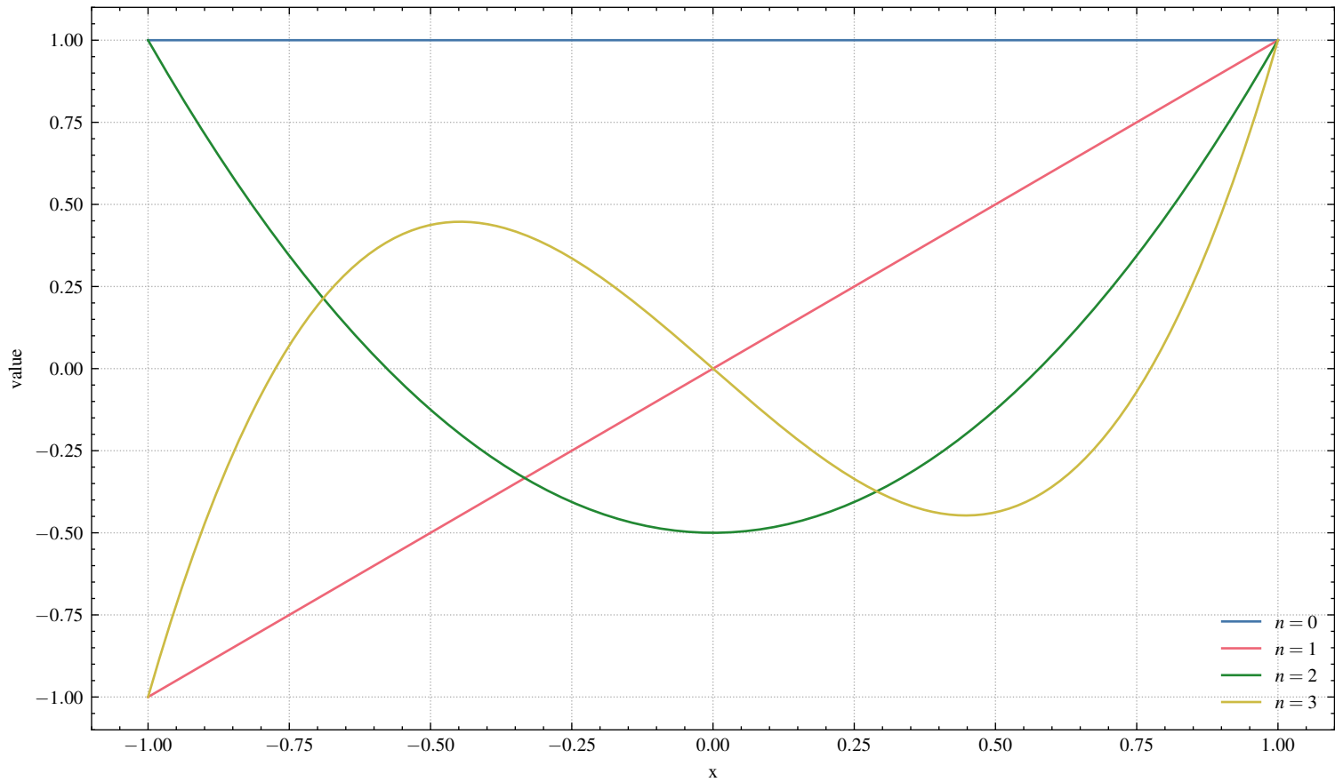
Jacobi polynomials (Legendre) P_n^{(0,0)}
