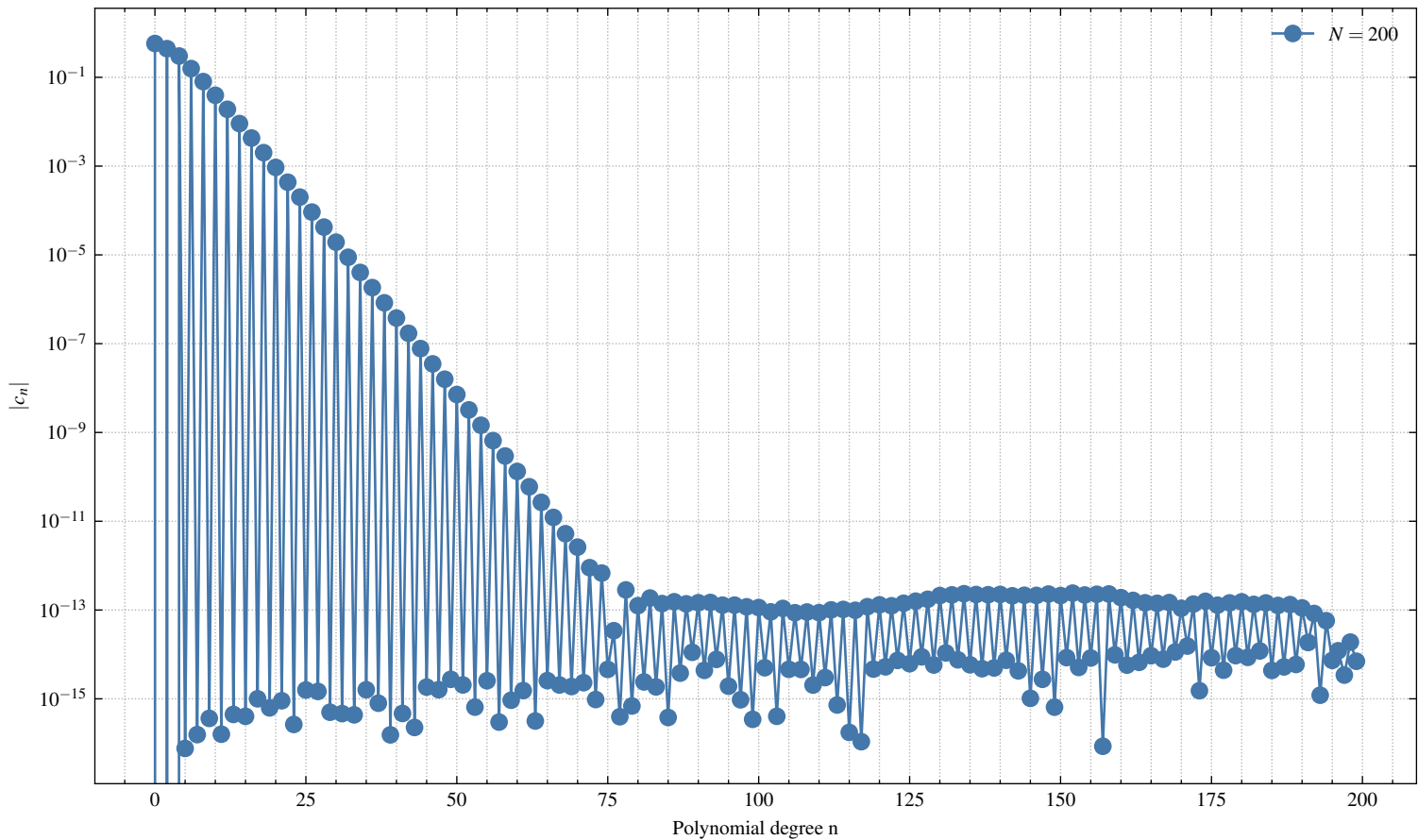
Legendre coefficients of u(x) = 1/(2 - \cos(\pi x))
