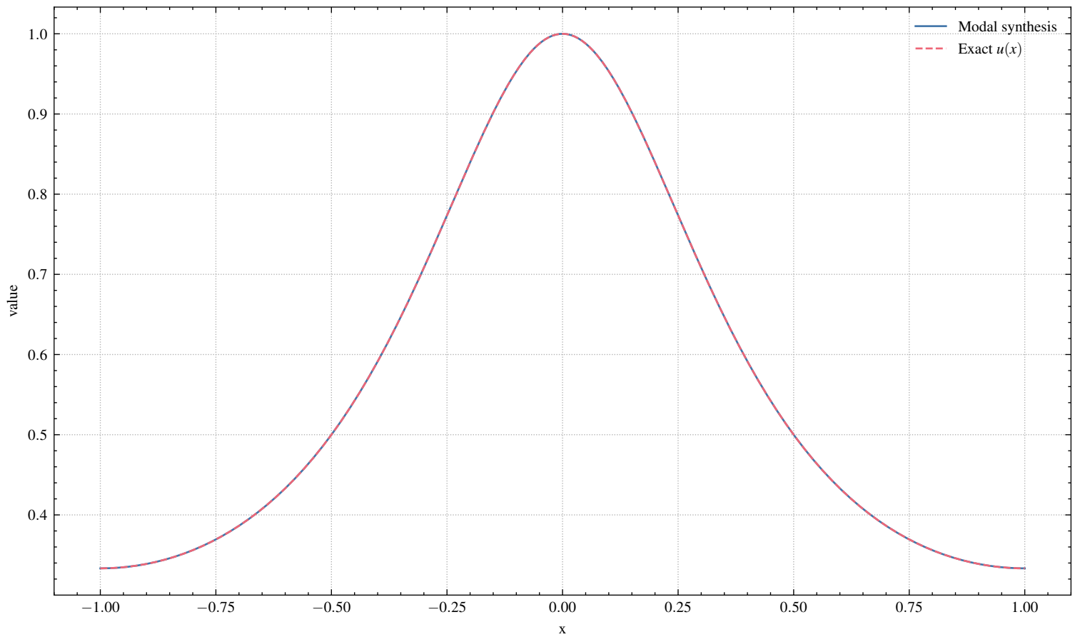
Legendre series reconstruction
