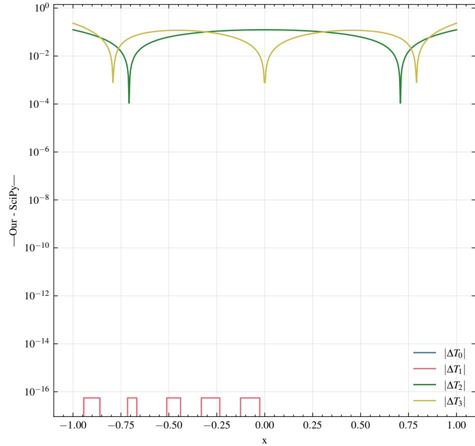
Absolute Difference (Chebyshev)
