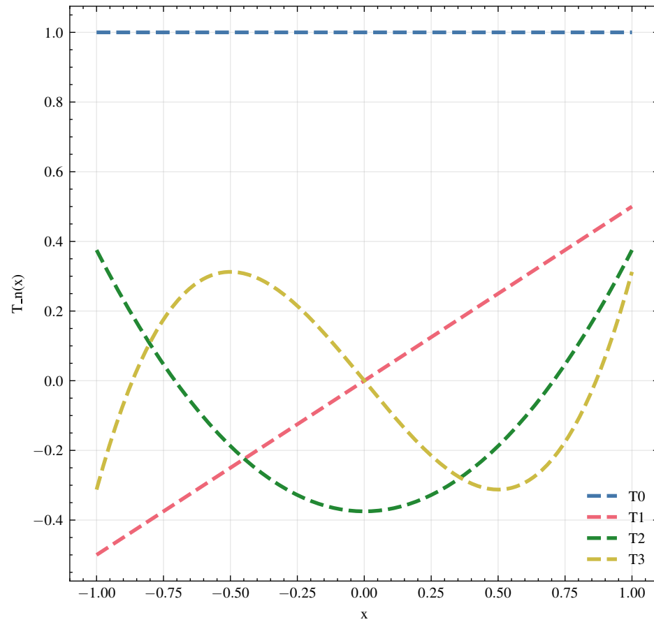
SciPy Implementation (Chebyshev)
