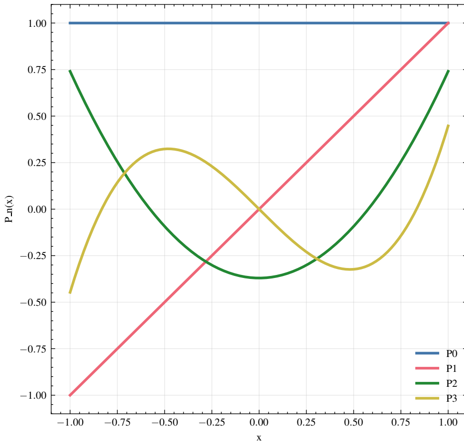
Our Implementation (Legendre)
