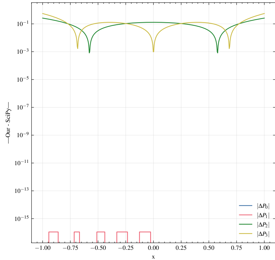
Absolute Difference (Legendre)
