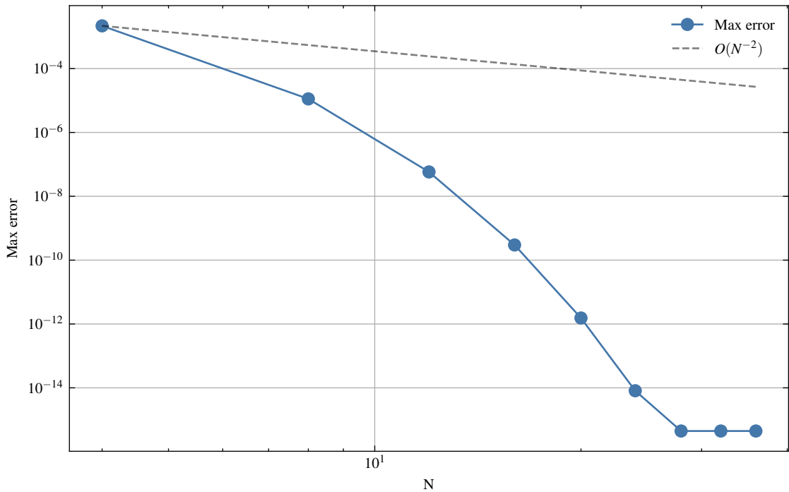
Max error vs N
