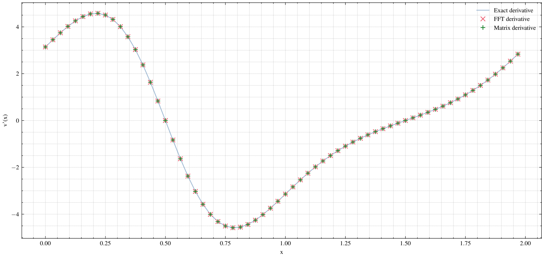
Spectral Differentiation: FFT vs Matrix vs Exact
