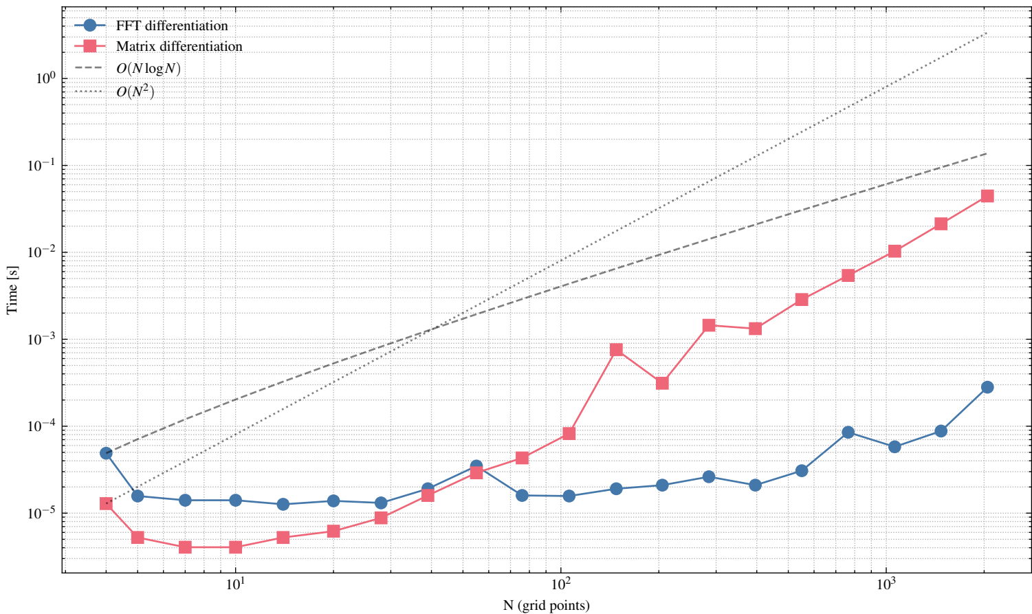
Performance: FFT vs Differentiation Matrix
