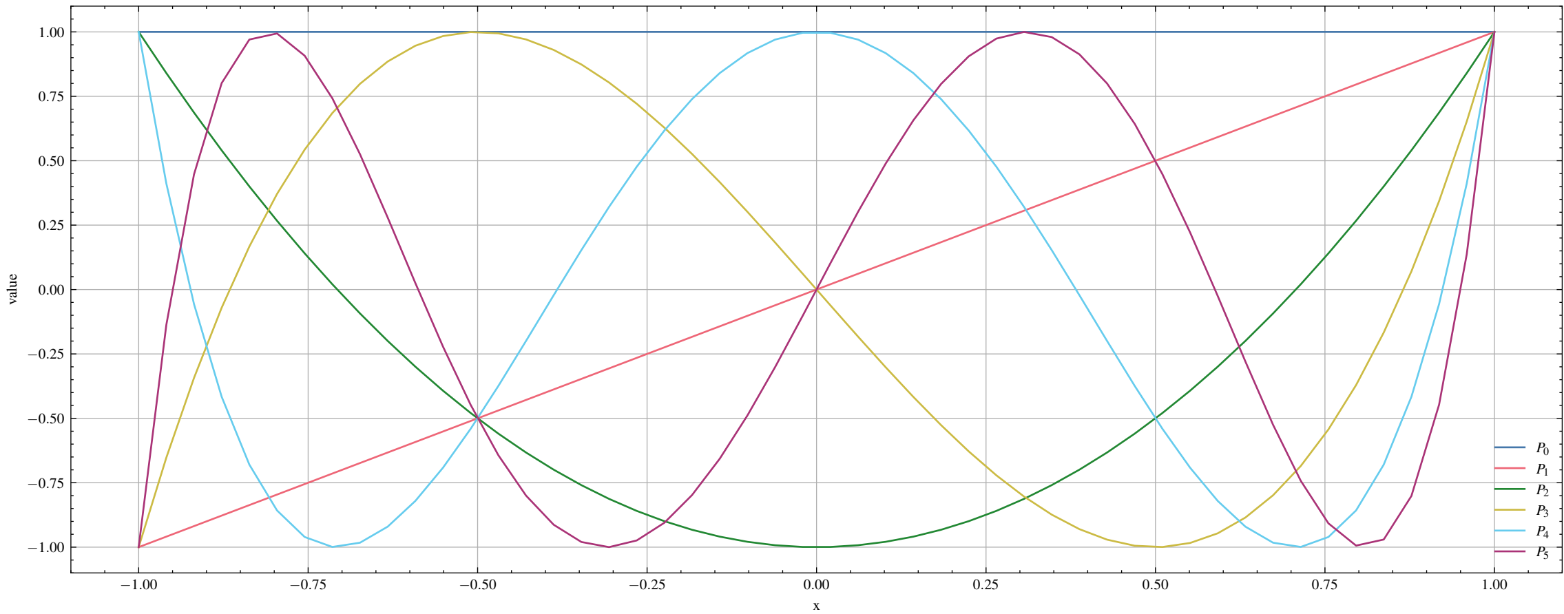
Chebyshev polynomials
