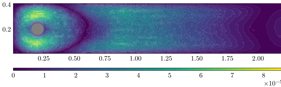
U Residual
