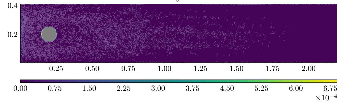
Continuity Residual
