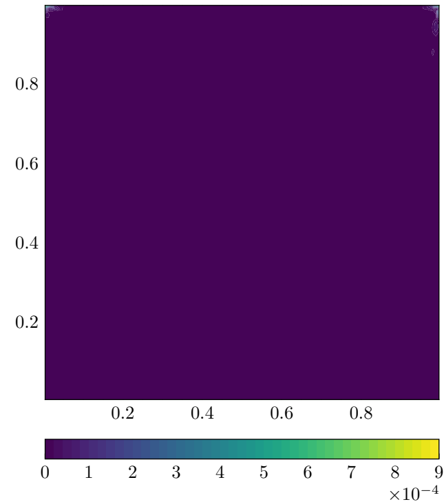
Continuity Residual
