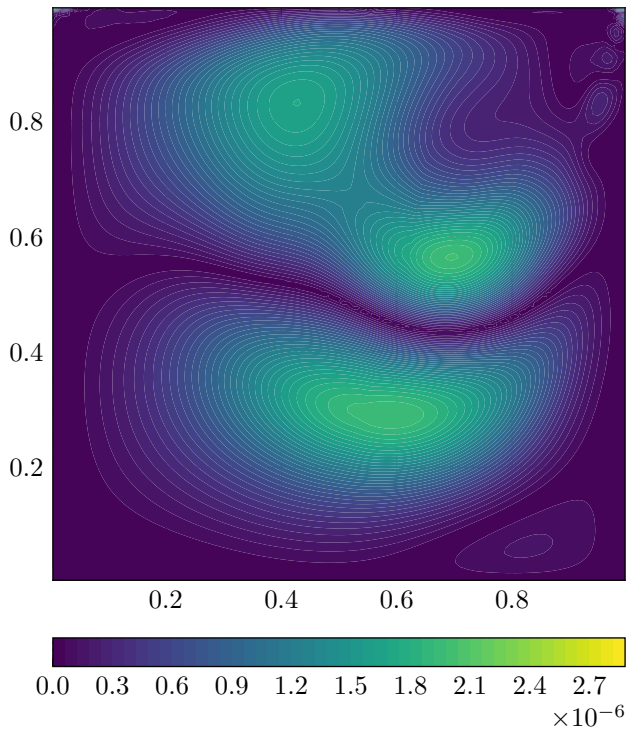
U Residual
