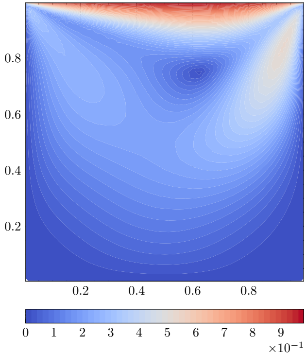
Velocity Magnitude
