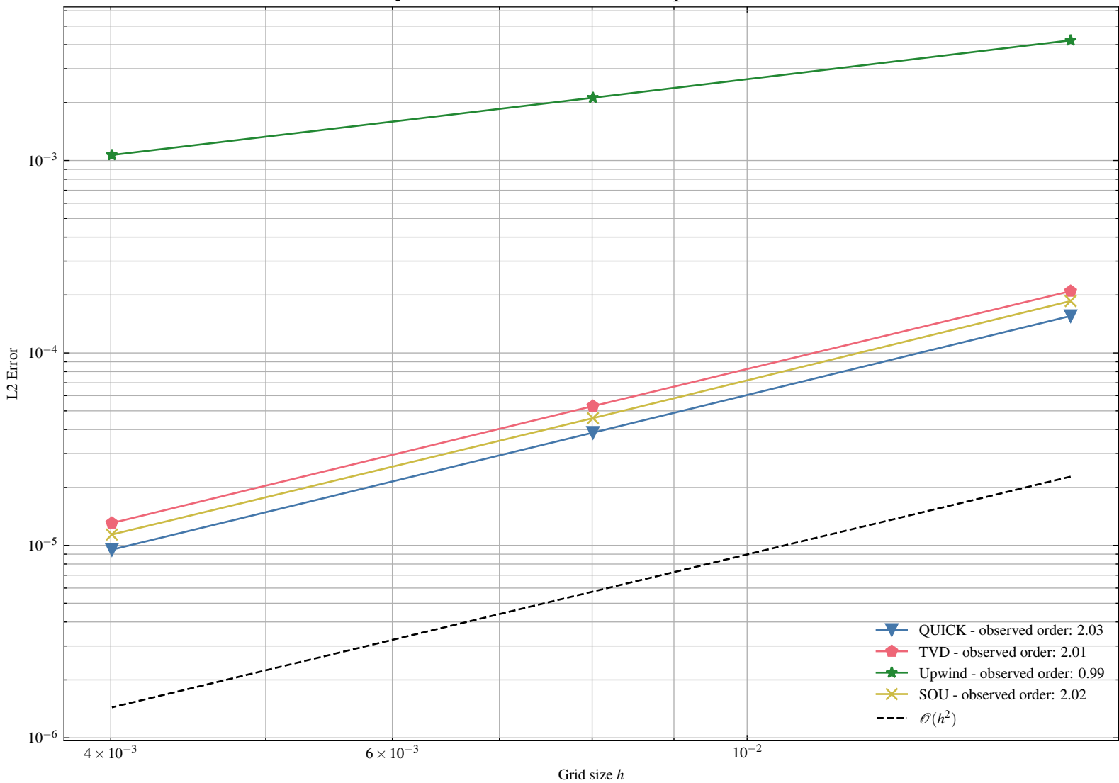
Order of Accuracy Convection-Diffusion Equation - Unstructured Mesh
