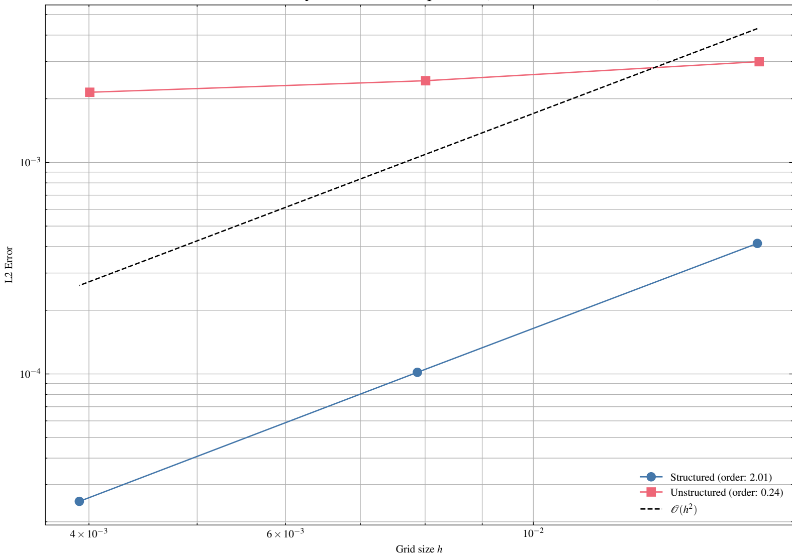
Order of Accuracy Poisson like equation (1 non-ortho correction)
