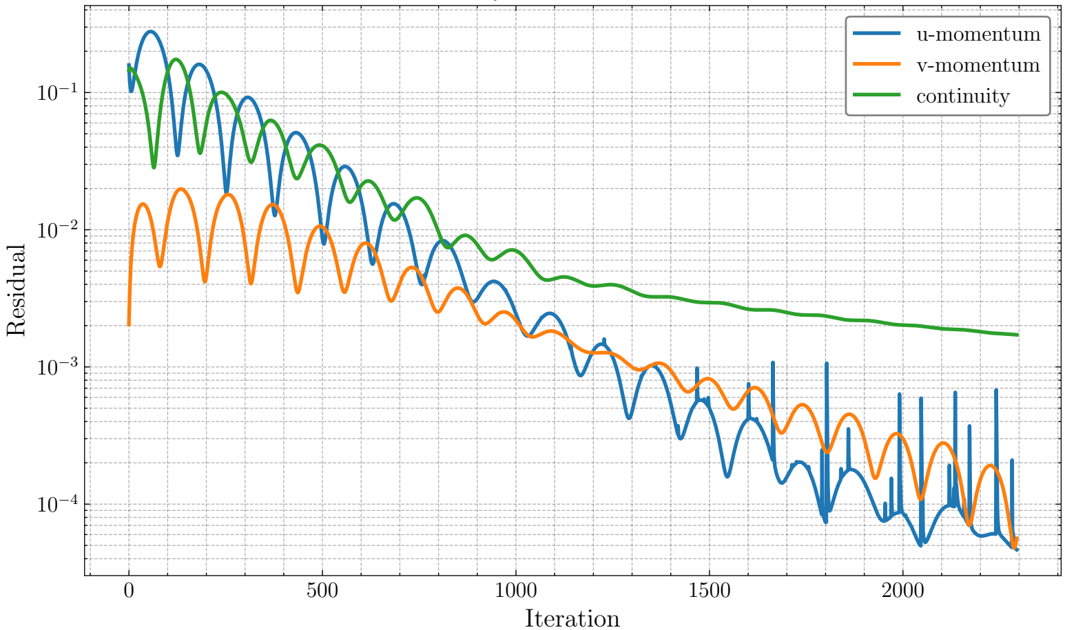
Residual History — Simulation ID: 2fafefd6
