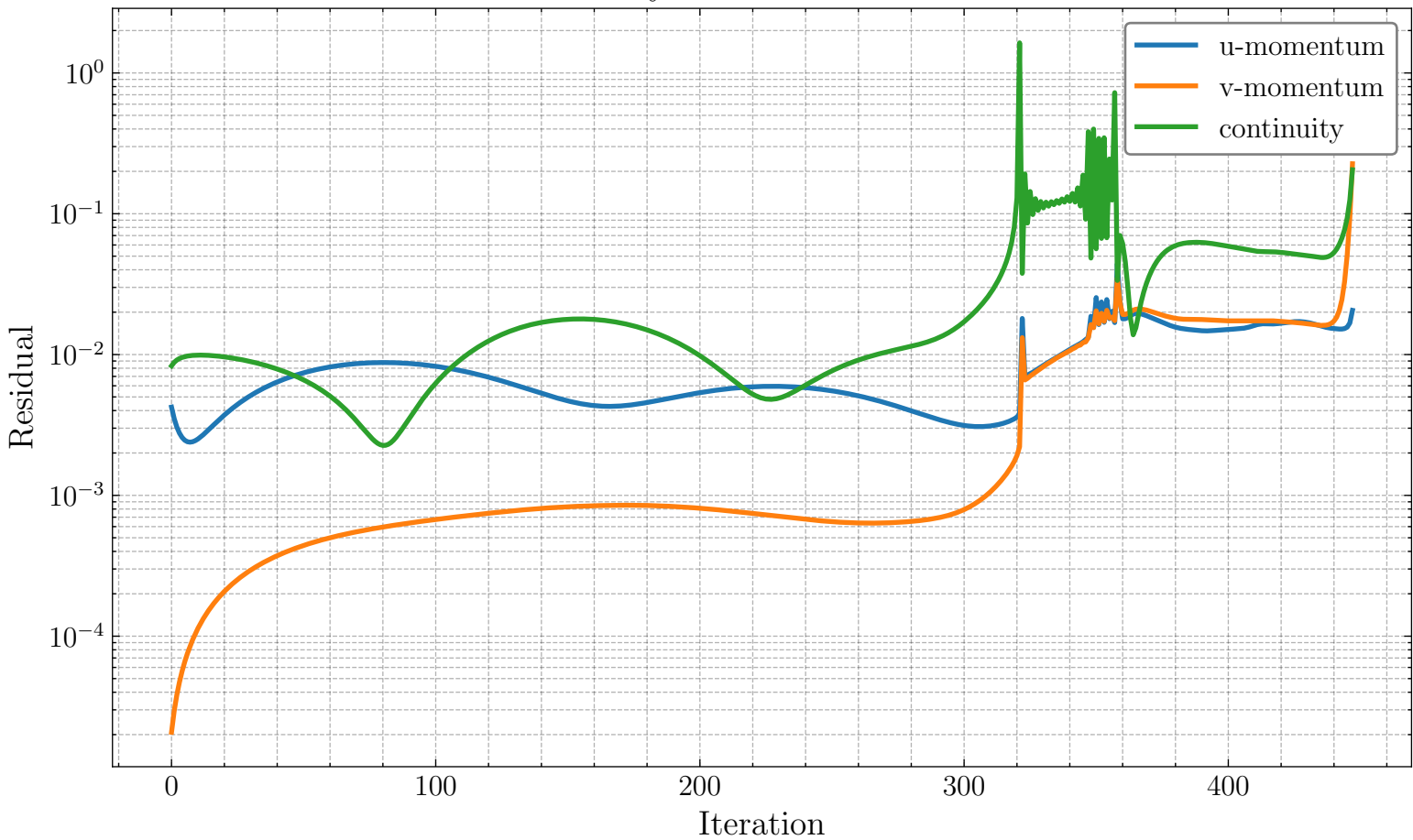
Residual History — Simulation ID: c4889f48
