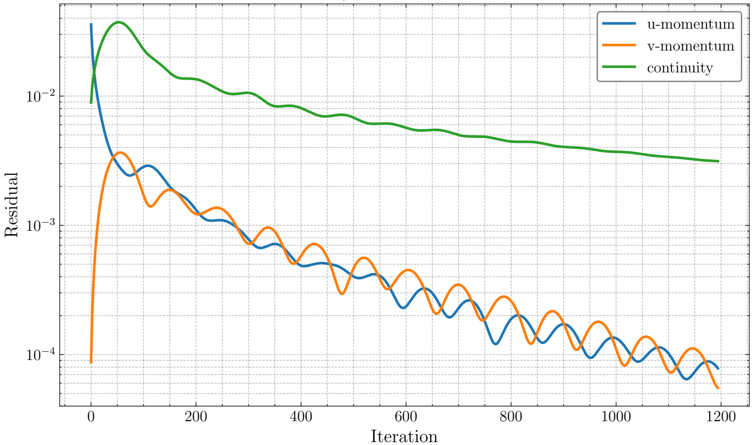
Residual History — Simulation ID: 2c1bb45e
