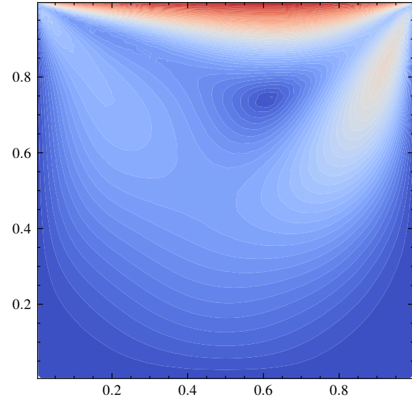
Velocity Magnitude
