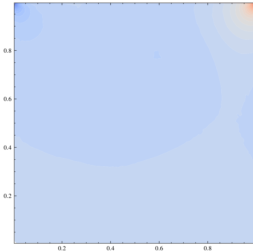
Pressure — Simulation ID: 1a61fd88
