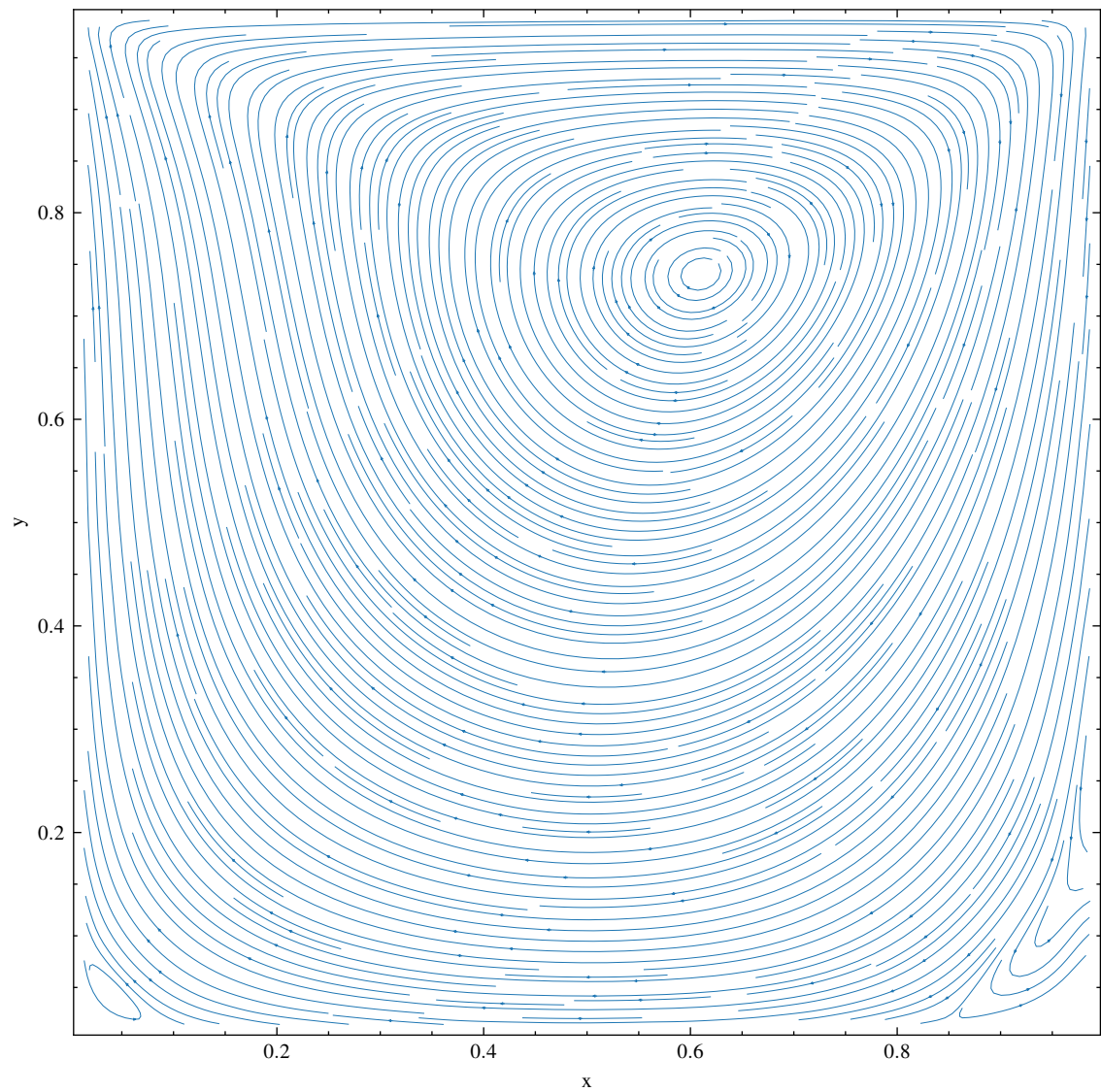
Streamlines — Simulation ID: 1a61fd88
