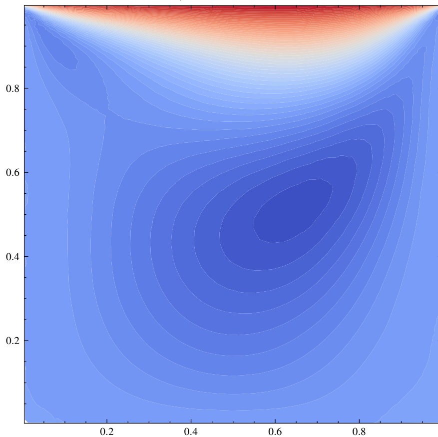
u-velocity — Simulation ID: 1a61fd88
