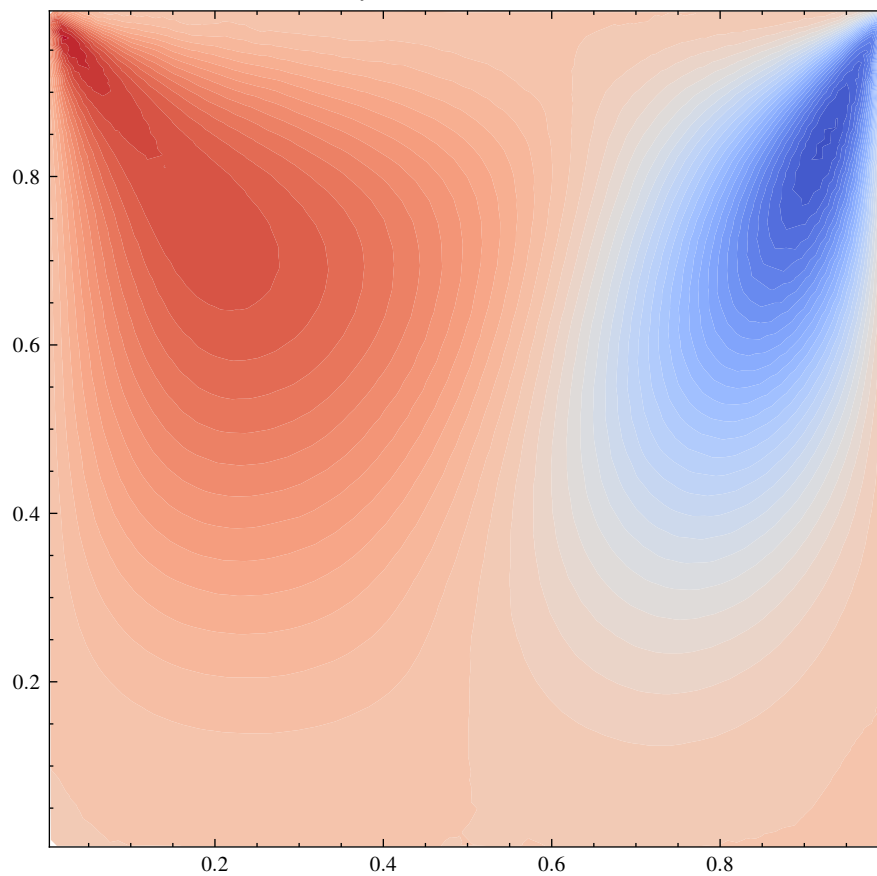
v-velocity — Simulation ID: 1a61fd88
