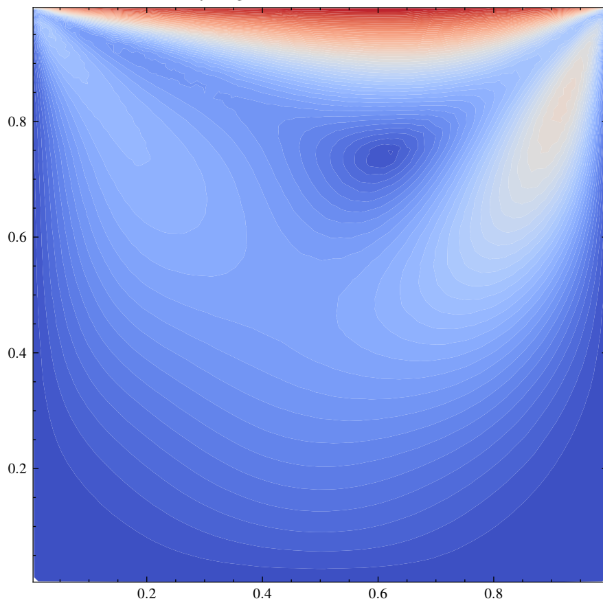
Velocity Magnitude — Simulation ID: 1a61fd88
