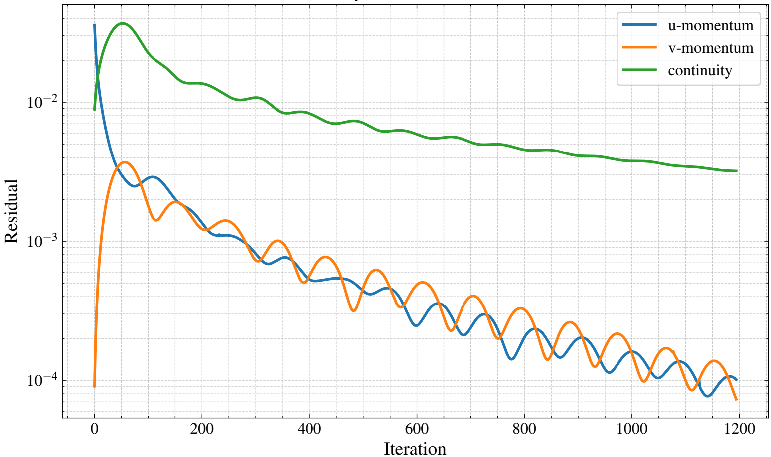
Residual History — Simulation ID: 1a61fd88
