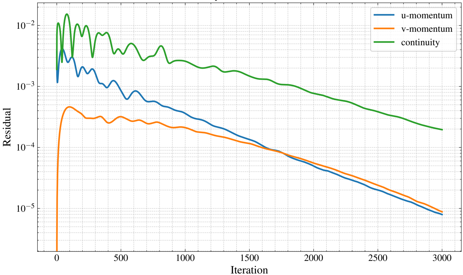
Residual History — Simulation ID: de9cadff
