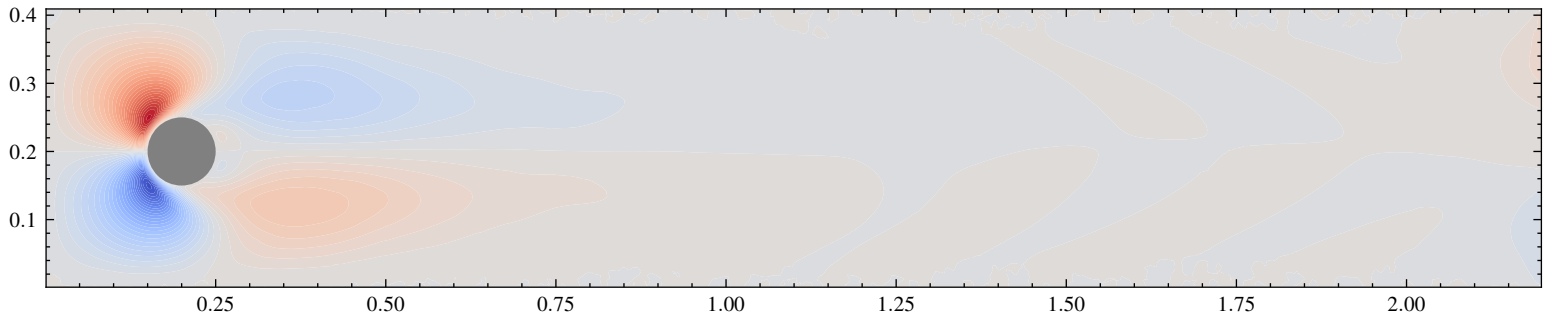
v-velocity — Simulation ID: de9cadff
