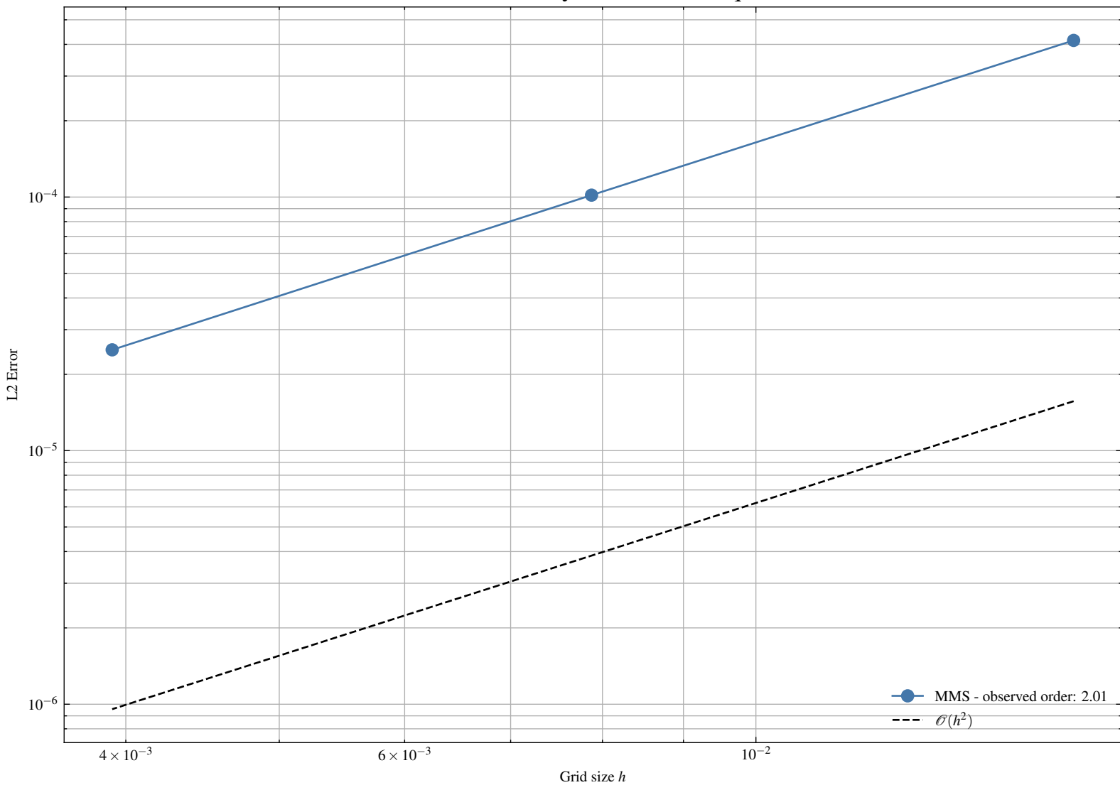
Order of Accuracy Poisson like equation
