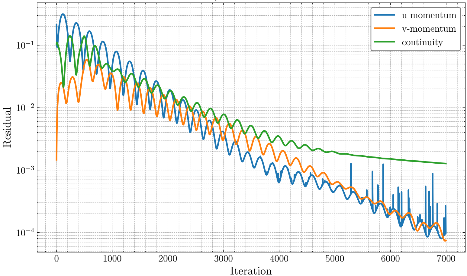
Residual History — Simulation ID: faf37ba2
