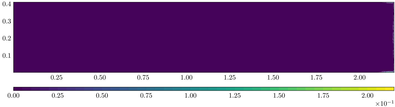
Continuity Residual — Simulation ID: 87456c36
