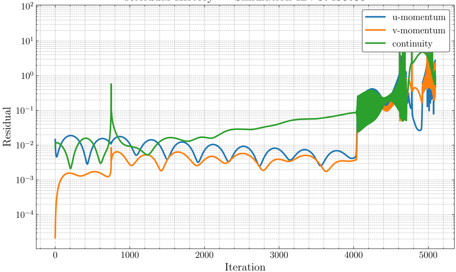
Residual History — Simulation ID: 87456c36
