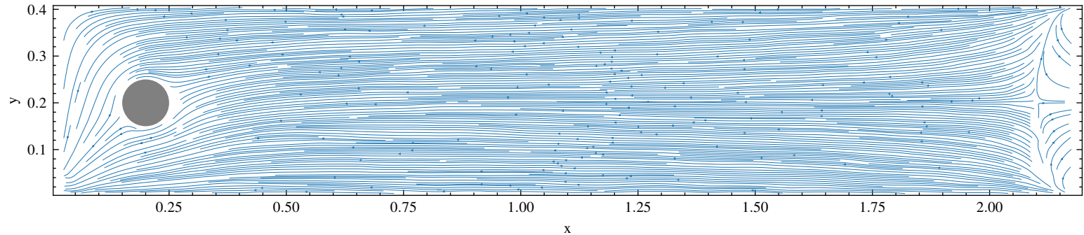
Streamlines — Simulation ID: 0a9cde15
