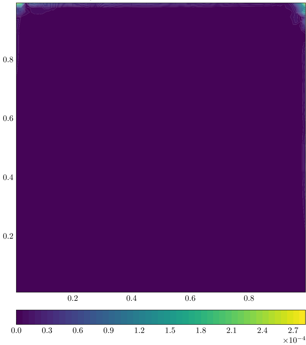
Continuity Residual — Simulation ID: 4f586c7b
