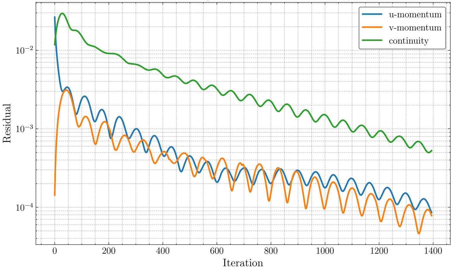
Residual History — Simulation ID: 4f586c7b
